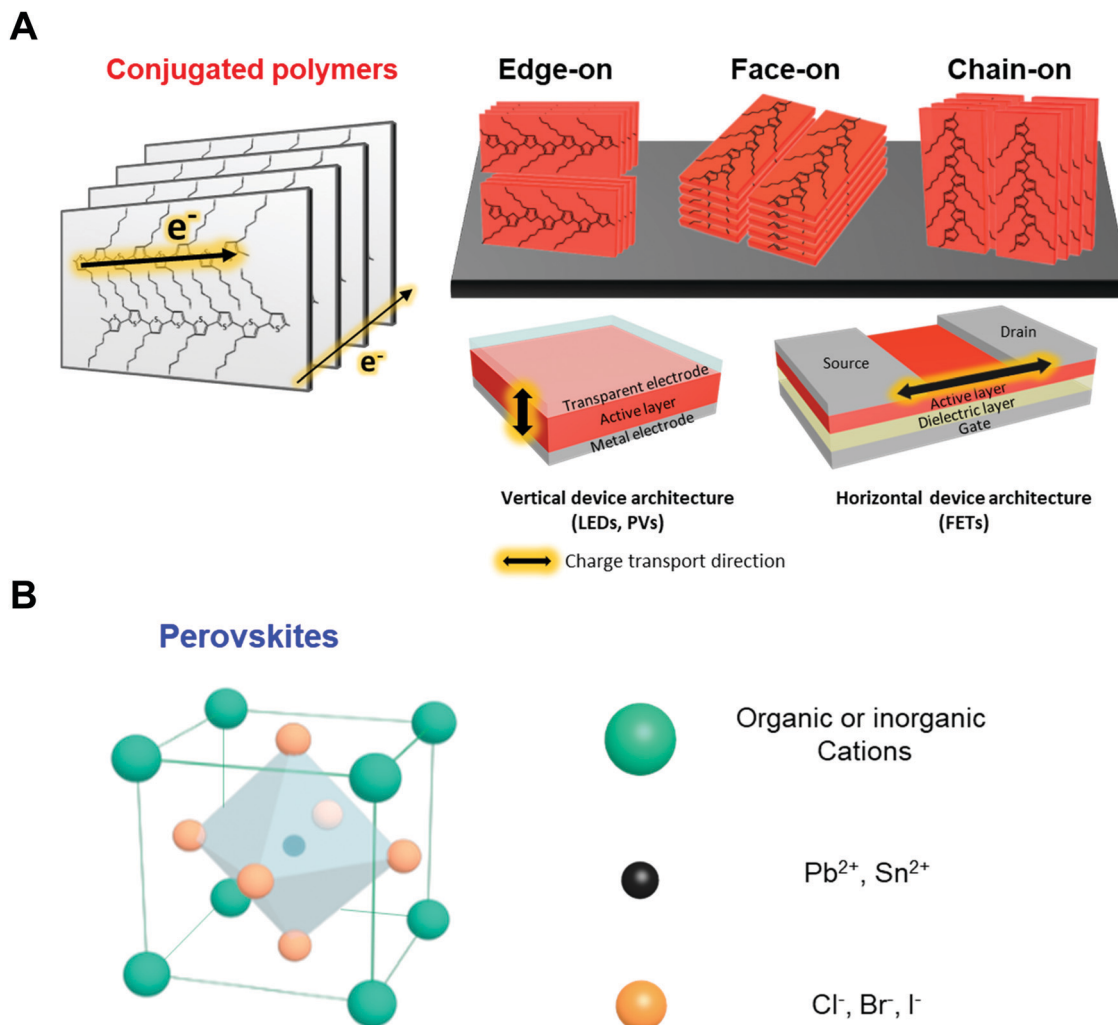
Fig. 2 Schematic illustration of solution-processable optoelectronic materials. (A) Structural representation of conjugated polymer (P3HT) with different molecular orientations (i.e., edge-on, face-on and chain-on orientation) for different directions of charge transport and their corresponding optoelectronic applications. (B) Structural representation of perovskite, \text{ABX}_3 where A is methylammonium (MA), formamidinium (FA) or Cs, B is Pb or Sn, and X is Cl, Br or I.
