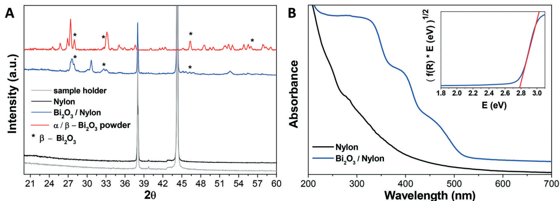
Fig. 2 A) XRD patterns of the sample holder, bare nylon, \text{Bi}_2\text{O}_3 /nylon composite, and synthesized \alpha/\beta\text{-Bi}_2\text{O}_3 powder, and B) UV-vis DRS spectra of bare nylon and \text{Bi}_2\text{O}_3 /nylon composite; inset: Tauc plot for the estimation of the bandgap.
