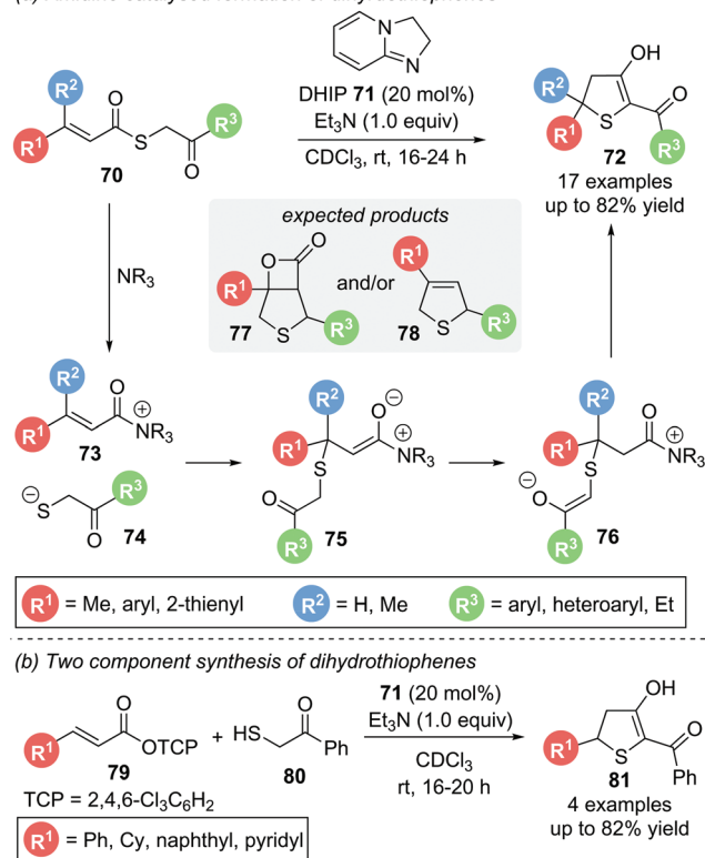
Scheme 14 Thia-Michael addition – Dieckmann cyclisation for the synthesis of dihydrothiophenes.
