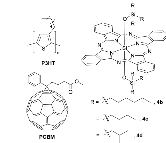
Fig. 7 Chemical structures of P3HT, PCBM and SiPc derivatives 4a–4c .
