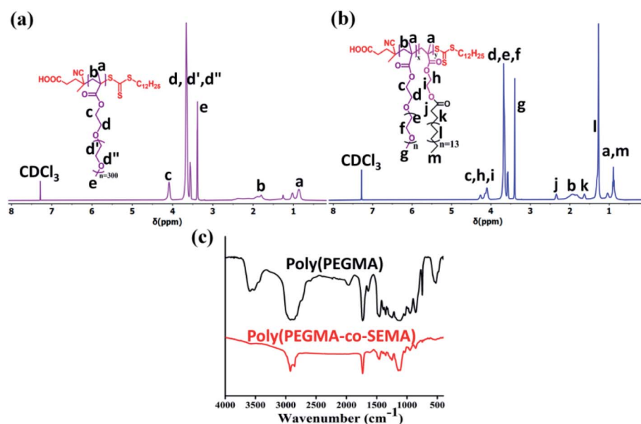
Fig. 2 ^1\text{H} NMR spectra of synthesized (a) poly(PEGMA) (b) poly(PEGMA-co-SEMA) (BCP50) polymer and (c) FTIR spectra of poly(PEGMA) and poly(PEGMA-co-SEMA) (BCP50) polymer.
