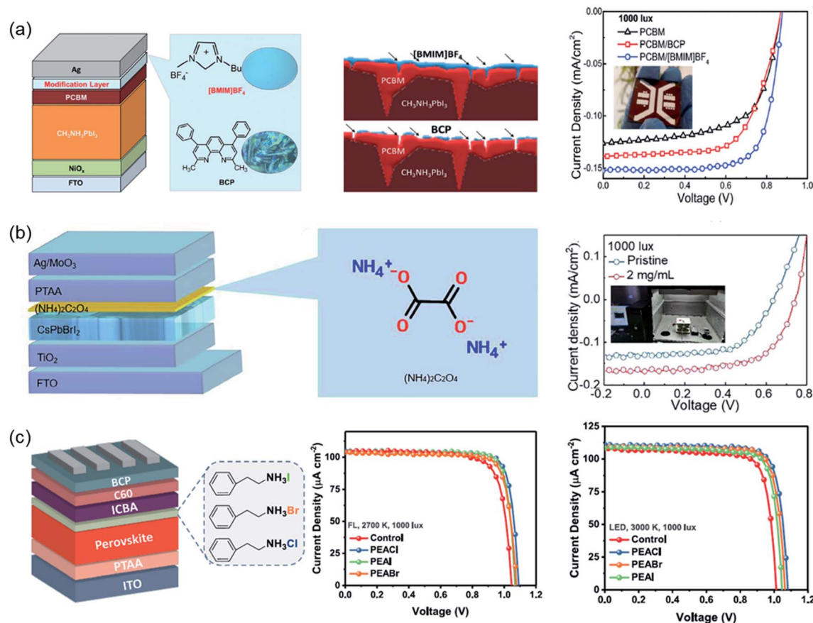
Fig. 6 (a) Inverted structure PSCs, molecular structure of [BMIM]BF 4 and BCP and the J - V curves. Reproduced from ref. 213 with permission from the [Wiley-VCH], copyright [2018]. (b) Device structure of CsPbBrI 2 based PSCs, molecular structure of (NH 4 ) 2 C 2 O 4 , and the J - V curves of devices with/without treatment. Reproduced from ref. 215 with permission from the [Elsevier], copyright [2020]. (c) Schematic diagram of PIPVs, the chemical structures of PEACl, PEABr, PEAI, and the J - V curves of the device with/without treatment under CFL and LED irradiation. Reproduced from ref. 216 with permission from the [Elsevier], copyright [2020].
