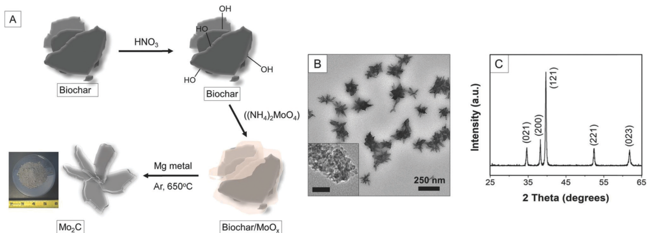
Fig. 63 (A) Schematic representation of synthesis of \text{Mo}_2\text{C} nanostructures. (B) TEM image (inset: scale bar = 25 nm) and (C) the powder XRD pattern of \text{Mo}_2\text{C} derived from biochar. Reproduced with permission from ref. 1002. Copyright Wiley 2018.
