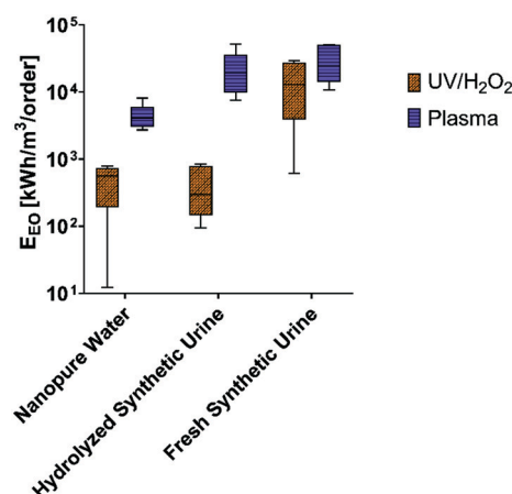
Fig. 4 Calculated electric energy per order ( E_{\text{EO}} ) (kW h m -3 per order) for both bench-scale reactors in the nanopure water and synthetic urine matrixes. The box and whisker plot displays 95% confidence intervals for E_{\text{EO}} values ( n = 6 , all pharmaceutical compounds in each data point).
