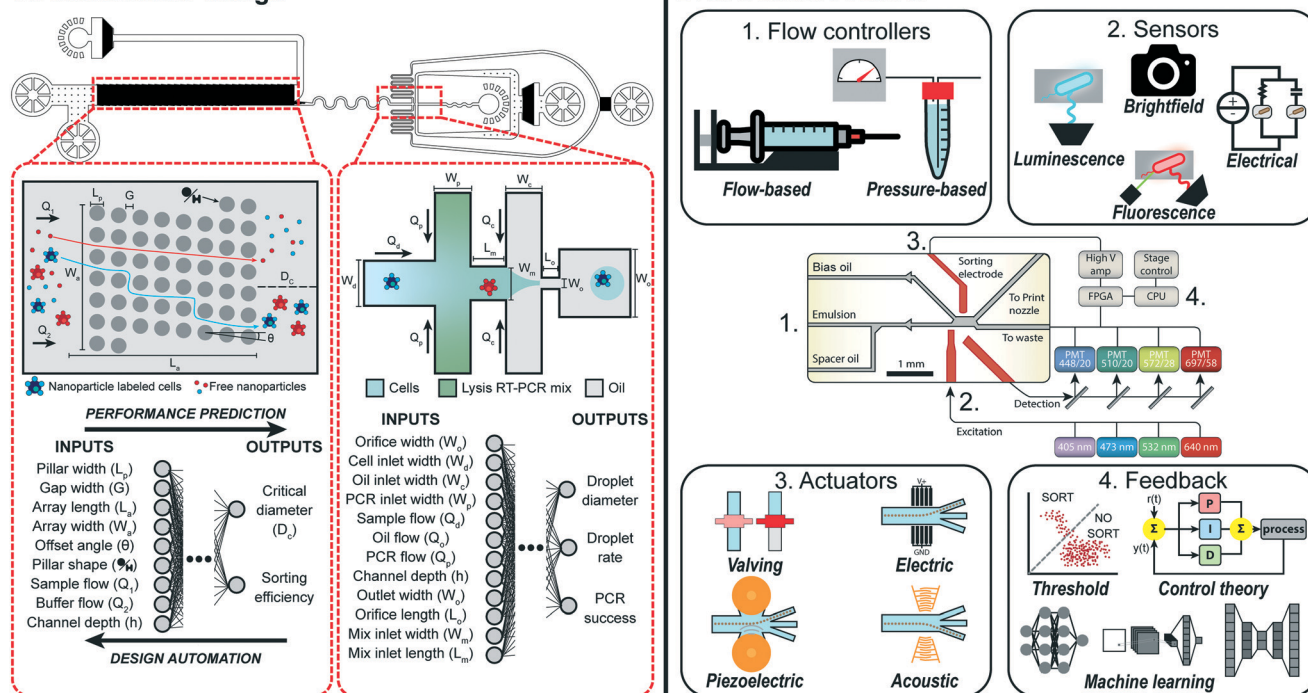
Fig. 1 Overview of machine learning enabled automated microfluidic design and control. (A) Complex microfluidic devices, such as the MATE-seq platform, 9 is comprised of two components, a deterministic-lateral-displacement array and droplet generator, which can be parameterized to describe both the physical design and experimental conditions. By mapping these parameters to a target performance, datasets can be generated and used to train machine learning models that predict the performance of each component. Design automation tools can use these models to automatically design each component such that the desired performance is achieved while adhering to design constraints. Figure reproduced from Ng et al. , 2019 (ref. 9) with permission from the Royal Society of Chemistry. (B) Microfluidic devices, such as a droplet sorter, can consist of a series of vital non-fluidic modules (schematic copyright 2017 National Academy of Sciences). 10 These include: (1) flow controllers to drive behavior of the device; (2) sensors to measure and quantify occurring phenomena; (3) actuators to manipulate device behavior on the single-event level; and (4) feedback systems to respond to sensor information and intelligently control device behavior via the other modules. Machine learning provides a sophisticated feedback system to intelligently link modules together to perform complex tasks in real-time.
