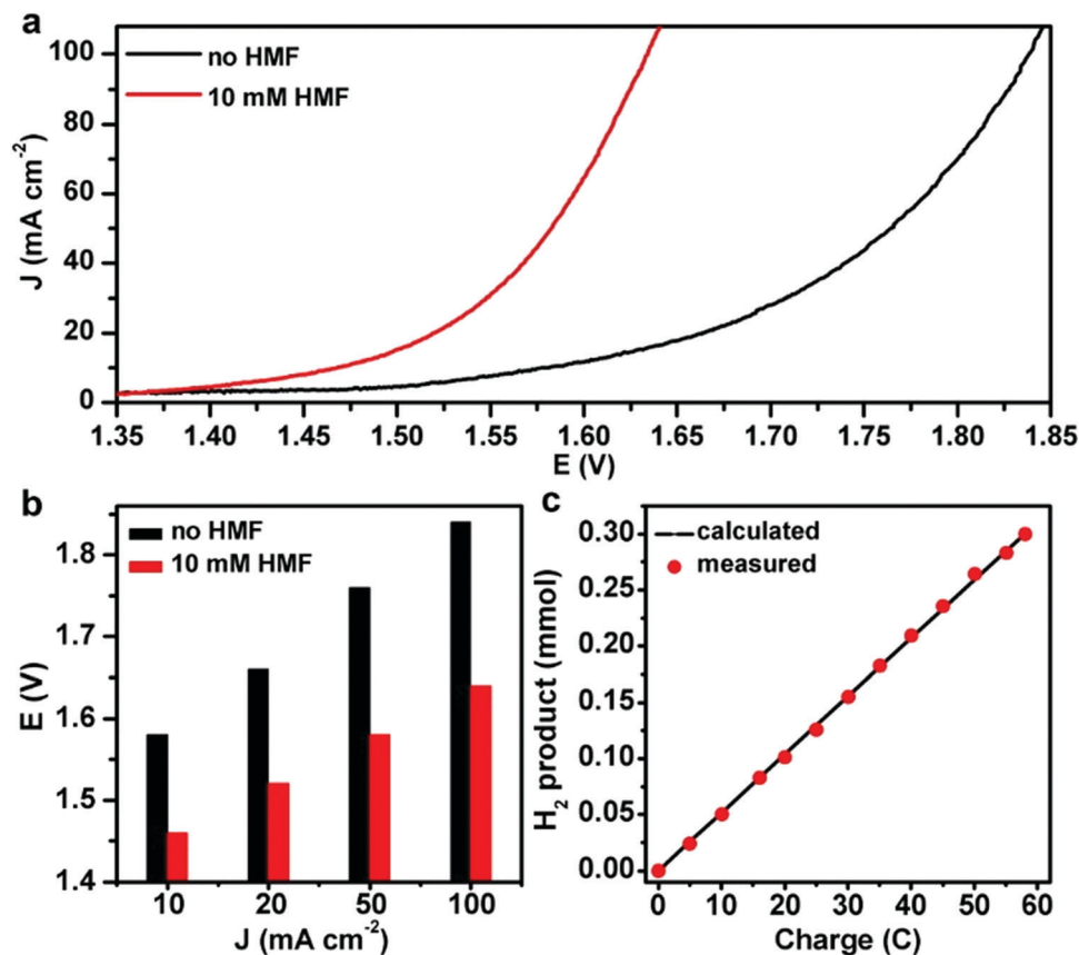
Fig. 17 (a) Two-electrode polarization curves and (b) comparison of the overpotentials to achieve benchmark current densities for the Ni_3S_2/NF couple in 1.0 M KOH with and without 10 mM HMF. (c) GC-measured H_2 quantity compared with theoretically calculated H_2 quantity assuming a 100% faradaic efficiency for the H_2 production catalysed by the Ni_3S_2/NF working cathode in 1.0 M KOH solution with 10 mM HMF. Reprinted with permission from ref. 300. Copyright 2016 American Chemical Society.
