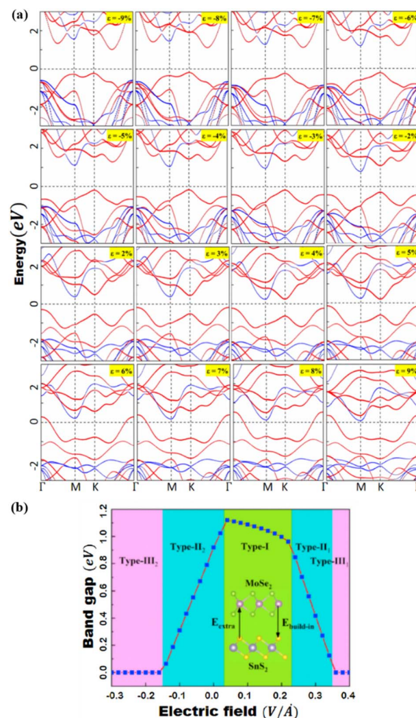
Fig. 9 (a) Under pressure, the band structures of MoSe 2 /SnS 2 heterostructures. MoSe 2 and SnS 2 are represented by the red and blue lines, respectively. (b) The bandgap of MoSe 2 /SnS 2 heterojunctions varies as the external E-field changes. Reprinted from ref. 20 with permission from Elsevier, copyright 2021.
