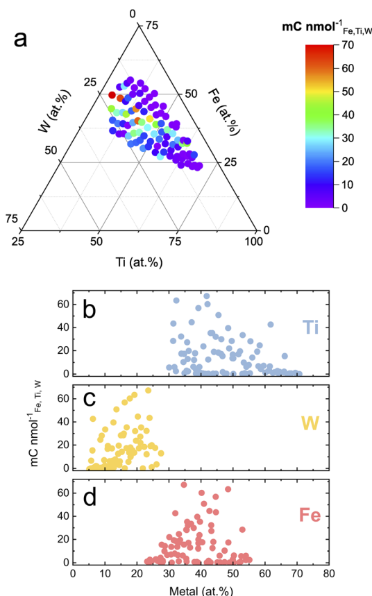
Fig. 3 Photocharge normalized by the total dissolution of the Fe–Ti–W–O material library measured at 1.7 V_{RHE} . (a) Dissolution-normalized photocharge mapped onto a ternary diagram. The performance metric is further plotted over the specific Ti (b), W (c), and Fe (d) content in the oxide films.
