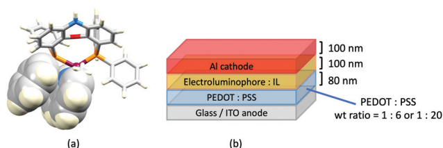
Fig. 19 (a) Structure of the cation in [Cu(HN-xantphos)(6-Mebpy)][PF_6] with the Ph \cdots bpy \pi -stacking interaction shown in space-filling representation (CSD refcode TUHXC). (b) Architecture of the LECs containing [Cu(BnN-xantphos)(6,6'-Me_2bpy)][PF_6] ; IL = [EMIM][PF 6 ], and Cu-ITMC: IL molar ratio = 4 : 1; two compositions of the hole-injection layer were used; LECs were driven using a pulsed current.
