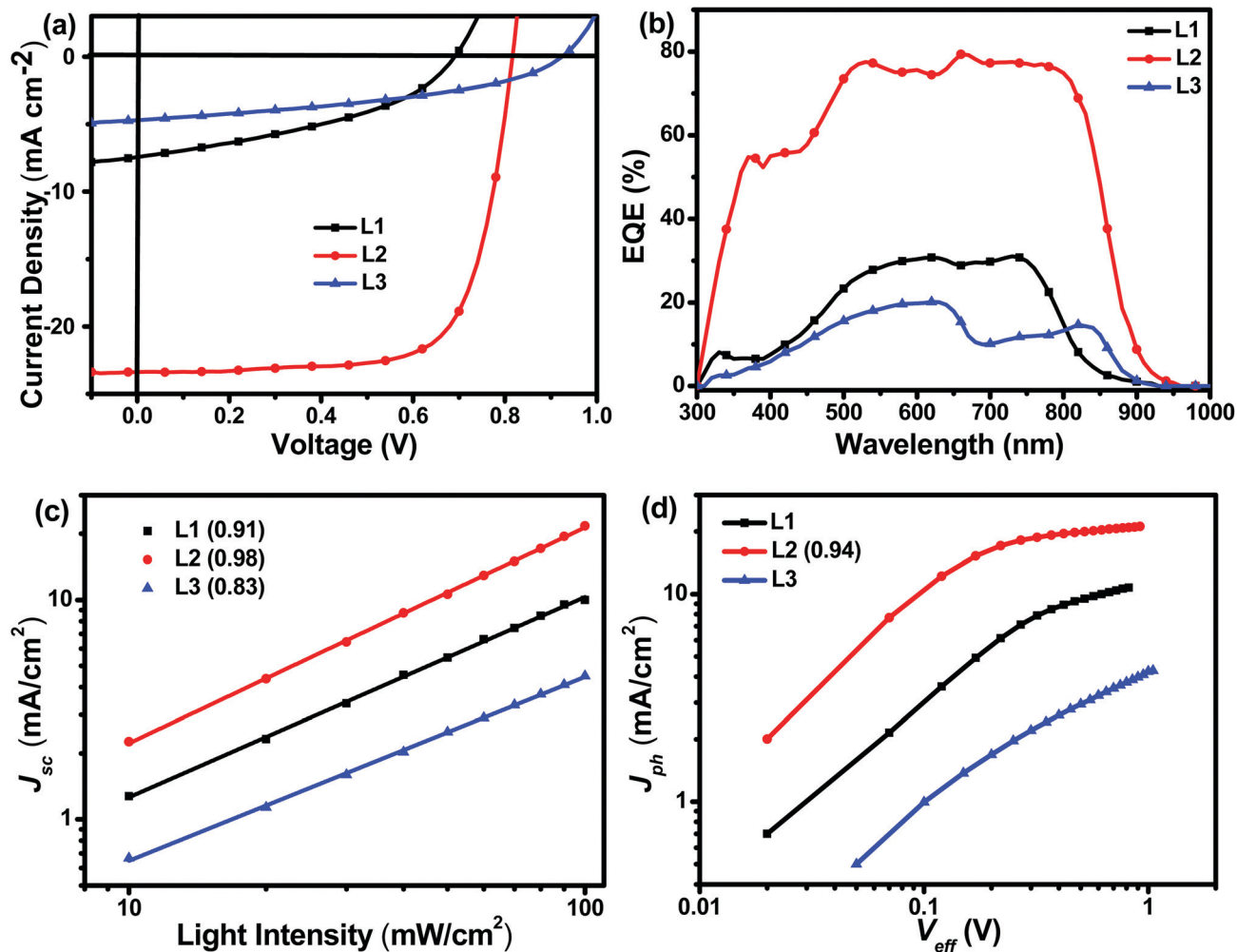
Fig. 3 (a) J - V and (b) EQE curves of L1-, L2-, and L3-based devices, (c) the dependence of J_{sc} on P_{\text{light}} and (d) the dependence of J_{ph} on V_{\text{eff}} .
