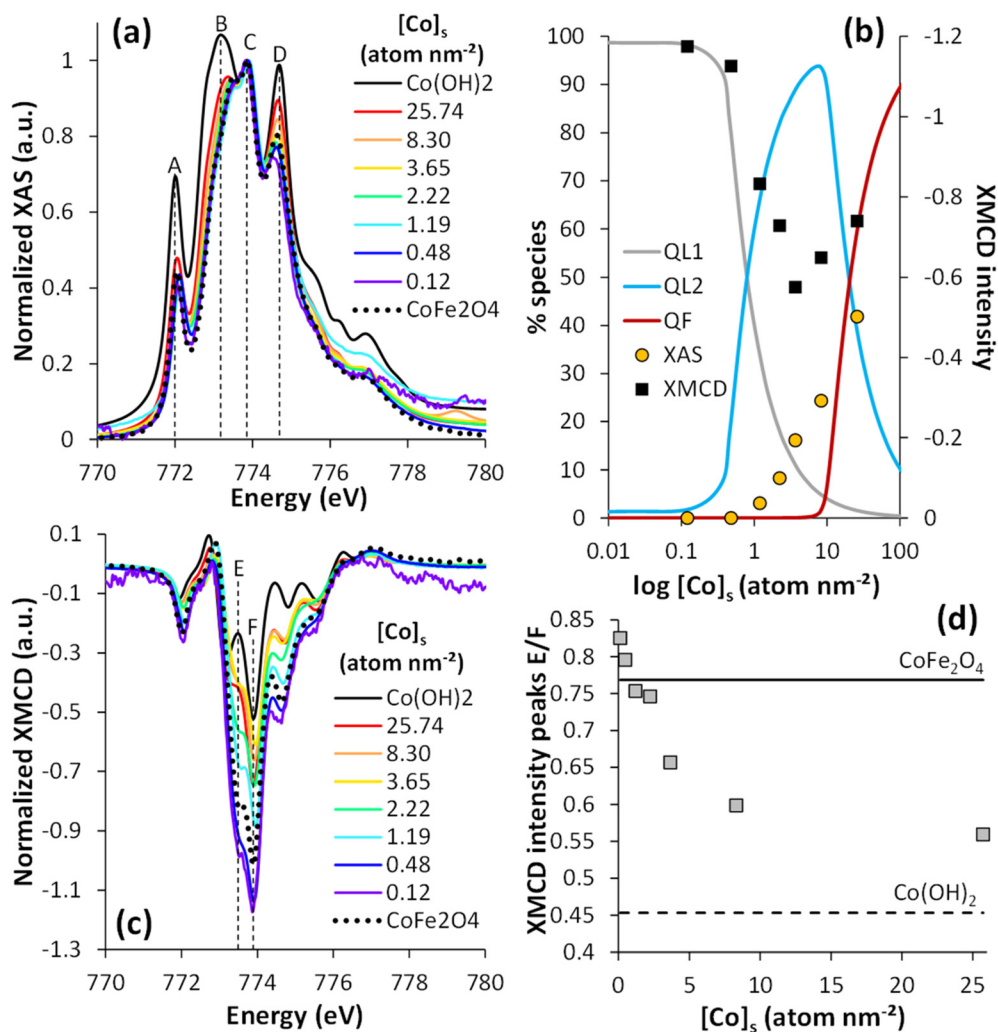
Fig. 2 Normalized XAS (a) and XMCD (c) spectra at the Co L_{3-} edge (see L_{2,3-} edges in Fig. S3†) of stoichiometric magnetite with different Co surface loadings ( 0.12 \leq [\text{Co}]_s \leq 25.74 atom per \text{nm}^2 ). XAS and XMCD signals were normalized by dividing the raw signal by the maximum XAS peak. (b) Percentage of the different species identified using the adsorption isotherm eqn (2) versus Co surface loading compared to the percentage of the \text{Co}(\text{OH})_{2(s)} -like phase calculated from LCF of XAS data (yellow points) and, on the secondary axis, the XMCD intensity (black squares). (d) XMCD intensity ratio of E and F peaks, as a function of [\text{Co}]_s . The dotted line corresponds to the XMCD intensity of \text{Co}(\text{OH})_{2(s)} and the solid line to \text{CoFe}_2\text{O}_4 references.
