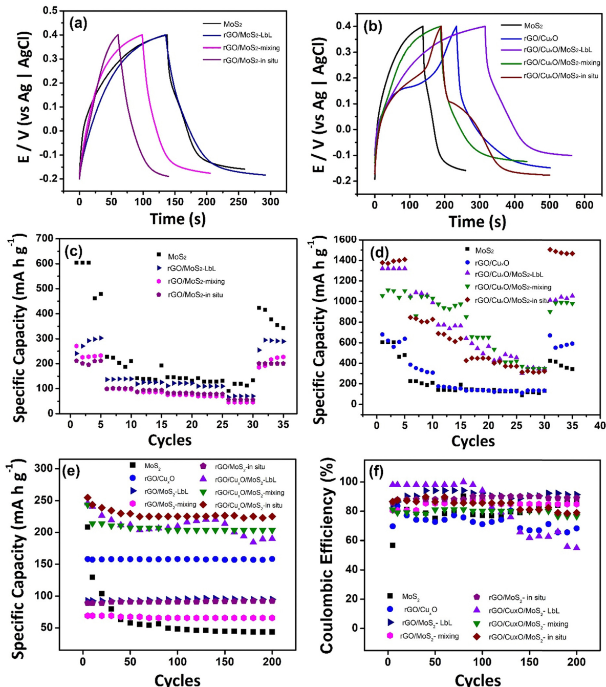
Fig. 8 Charge and discharge curves (a) and (b); specific capacity of the discharge process (c) and (d) at different current densities (0.1, 0.25, 0.5, 0.75, 1 and 2 A g -1 ); specific capacity measured during 200 cycles at 2 A g -1 (e) and Coulombic efficiency (f) of the nanocomposites in 0.1 mol L -1 NaCl aqueous solution and the potential range of -0.2 to 0.4 V.
