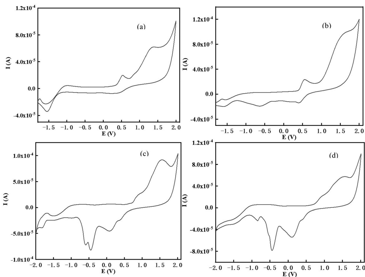
Fig. 6 Cyclic voltammograms of the chalcones in DCM against saturated calomel electrode (SCE) under a nitrogen saturated atmosphere, (a) TPA-1; (b) TPA-2; (c) DFO-1; (d) DFO-2.
