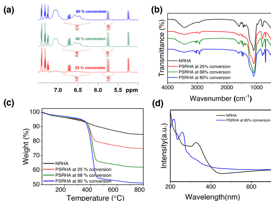
Fig. 3 (a) Conversion of three different reactions was determined using ^1\text{H} NMR spectroscopy with respect to the area under the vinyl proton of styrene observed at \delta = 5.7 ppm to the broad peak corresponding to the aromatic proton of polystyrene observed at \delta = 6.5 ppm. The conversions obtained are 25%, 68% and 80%. (b) FTIR spectra of polystyrene grafted on nitron functionalized RHA (NRHA) silica using ESCP (PSRHA) at 25%, 68% and 80% conversions. The intensity of the bands corresponding to the aromatic C–H stretching at 3022\text{ cm}^{-1} and out of plane C–H bending at 694\text{ cm}^{-1} was observed to increase with an increase of polystyrene grafting. (c) TGA plots for polystyrene grafted nitron functionalized RHA (NRHA) silica synthesized using ESCP (PSRHA) at 25%, 68%, and 80% conversion and the weight loss corresponding to the grafted polystyrene was observed to increase with an increase in conversion, which corresponds to the increased polystyrene grafting. (d) Solid-state UV-visible spectra of nitron functionalized RHA (NRHA) silica and polystyrene grafted silica synthesized using ESCP (PSRHA) at 80% conversion. The band corresponding to the nitron functionality was observed to decrease upon polymer grafting.
