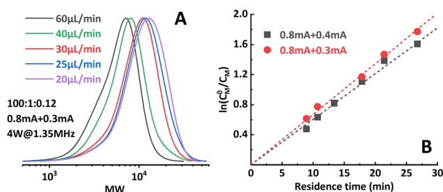
Fig. 4 (A) Molecular weight evolution of poly(methyl acrylate) synthesized by the two-reactor setup. (B) Good linearity of the first-order kinetic plot when proper i_{app} combinations were selected.
