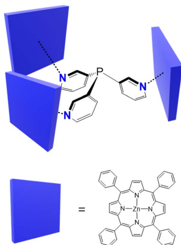
Fig. 1 First example of a \{[P(3\text{-py})_3] \cdot (ZnTPP)_3\} assembly.
