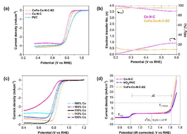
Fig. 5 (a) The LSV scans of the ORR in \text{O}_2 -saturated 0.10 M KOH solution at 1600 rpm. (b) electron transfer number and percentage of \text{HO}_2^- . (c) the LSV scans of the ORR at different loadings of Co in X% Co-ZIF ( X = 100, 110, 115 and 120\% ) in \text{O}_2 -saturated 0.10 M KOH solution at 1600 rpm. (d) overall polarization curves of optimal CoFe-Co-N-C, (ZIF-67-derived) Co-N-C and commercial Pt/C and \text{IrO}_2 in 0.1 M KOH.
