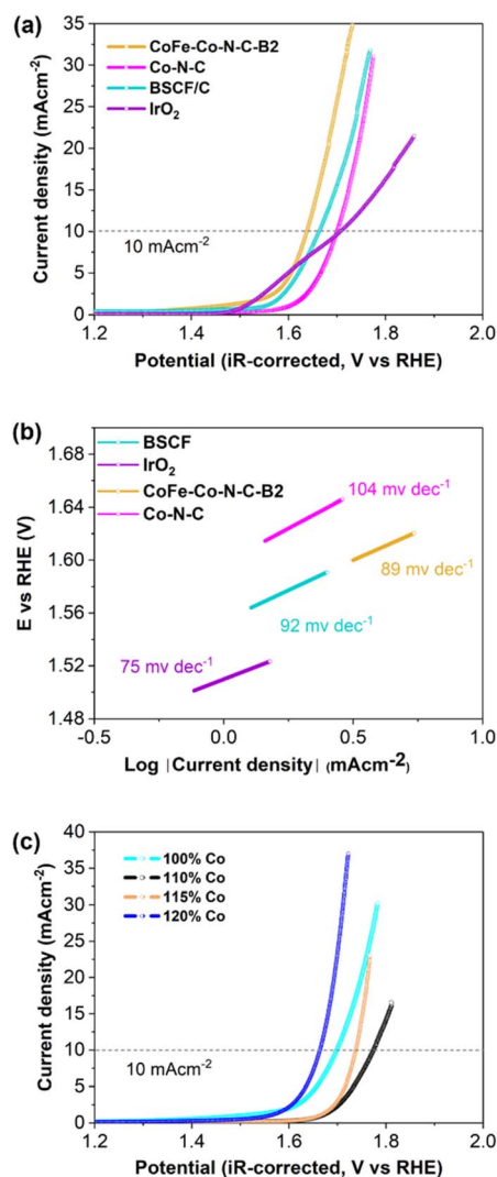
Fig. 4 (a) iR-corrected LSV curves of the OER in \text{O}_2 -saturated 0.10 M KOH solution at 1600 rpm; and (b) corresponding Tafel slopes. (c) iR-corrected LSV curves of the OER for different loadings of Co in X% Co-ZIF ( X = 100, 110, 115 and 120\% ) in \text{O}_2 -saturated 0.10 M KOH solution at 1600 rpm.
