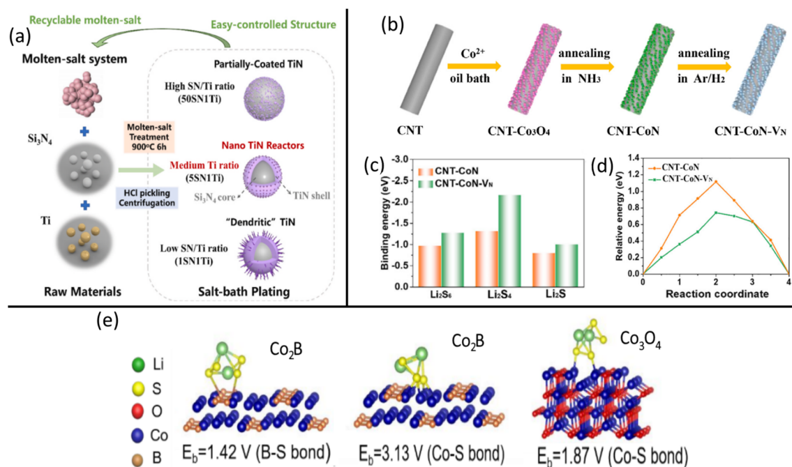
Fig. 14 (a) Schematic of a molten-salt process for synthesizing TiN/Si 3 N 4 core/shell structures with dendritic TiN 327 (Reproduced with permission from ref. 327. Copyright 2023, Elsevier). (b) Schematic illustrating the synthesis of nitrogen-vacant CoN (CoN-Vs) grown on CNT to yield CNT-CoN-Vs. (c) Binding energies of \text{Li}_2\text{S}_6 , \text{Li}_2\text{S}_4 , and \text{Li}_2\text{S} on pristine and nitrogen-vacant CoN/CNTs. (d) Diffusion energy barriers of \text{Li}_2\text{S} on pristine and nitrogen-vacant CoN/CNTs. 227 (Reproduced with permission from ref. 227. Copyright 2022, Elsevier). (e) Binding energies of \text{Li}_2\text{S}_4 on \text{Co}_2\text{B} with boron and cobalt sites, and the binding energy of \text{Li}_2\text{S}_4 on \text{Co}_3\text{O}_4 . 333 (Reproduced with permission from ref. 333. Copyright 2019, American Chemical Society).
