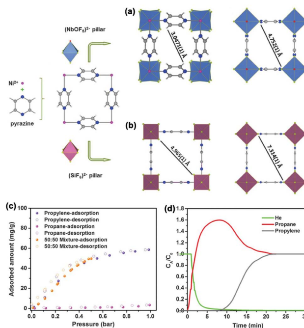
Fig. 11 Comparison of the building block arrangement of (a) KAUST-7 and (b) SIFSIX-3-Ni. (c) Adsorption isotherms of \text{C}_3\text{H}_6 , \text{C}_3\text{H}_8 , and an equimolar mixture of \text{C}_3\text{H}_6/\text{C}_3\text{H}_8 on KAUST-7 at 298 K. (d) Breakthrough curves for an equimolar \text{C}_3\text{H}_6/\text{C}_3\text{H}_8 mixture on KAUST-7 at 298 K. Reproduced from ref. 64 with permission from copyright 2016, The American Association for the Advancement of Science.
