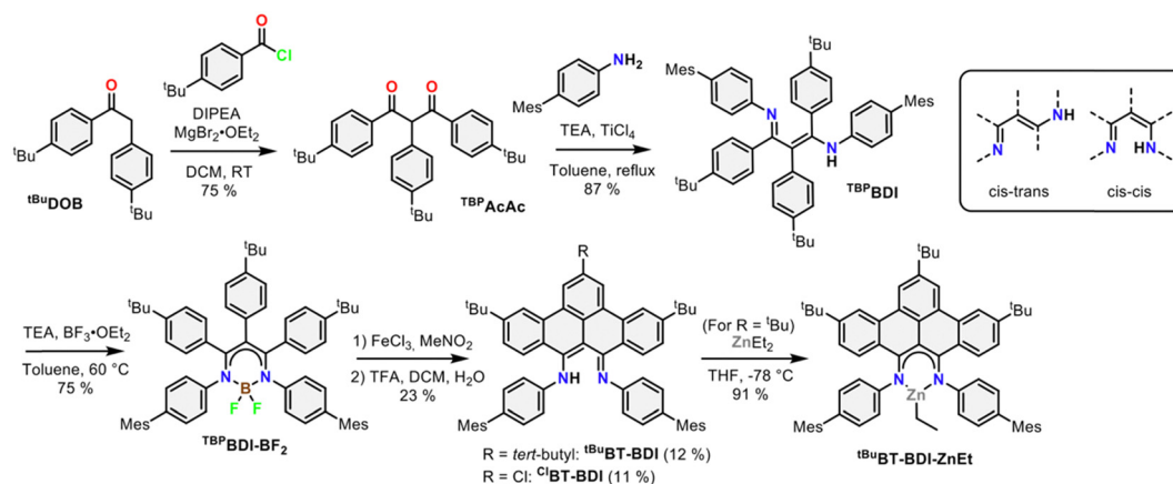
Scheme 1 Synthetic route towards BT-BDI and its ZnEt complex.
