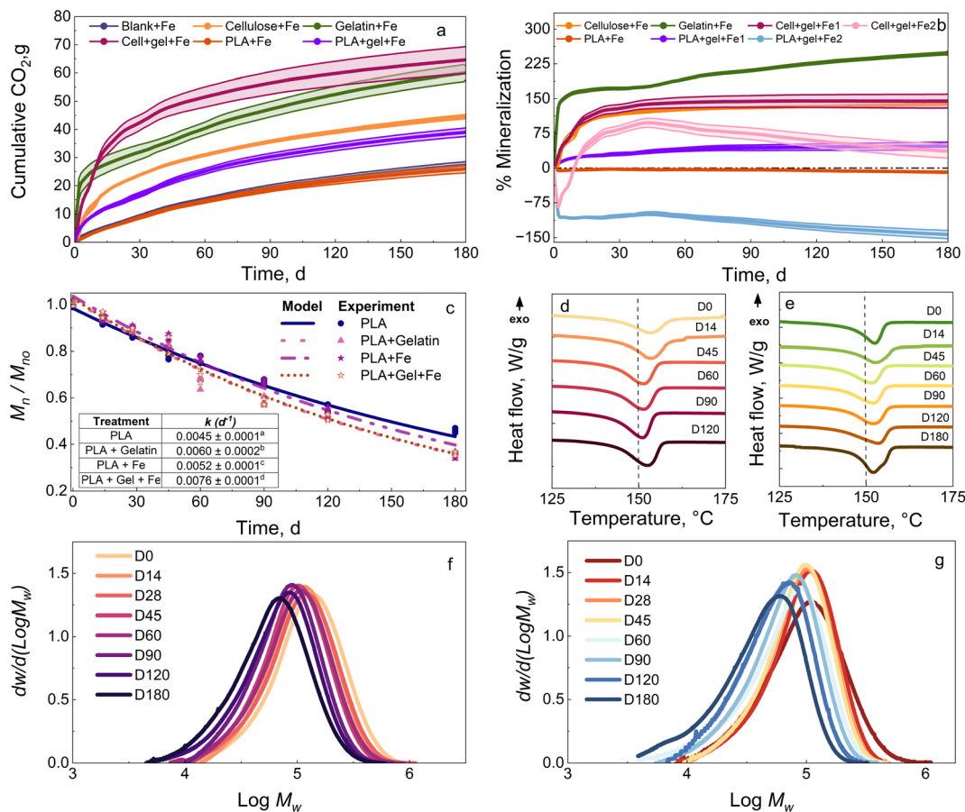
Fig. 3 Cumulative CO 2 evolution (a) and mineralization (b) of blank + Fe, cellulose + Fe, PLA + Fe, cellulose + gelatin + Fe, cellulose + gelatin + Fe (Cell + gel + Fe), PLA + gelatin + Fe (PLA + gel + Fe) in compost at 37 °C. (c) Represents the normalized M_n reduction as a function of time for PLA in control compost and compost biostimulated with gelatin, and gelatin + Fe. The experimental data was fitted using a first-order reaction of the form M_n/M_{no} = e^{-kt} , where M_{no} is the initial M_n , k is the rate constant, and t is the time. The inset shows the k -fitted values; values with different lowercase letters are statistically different ( \alpha = 0.05 , Tukey–Kramer test). (d) and (e) depict DSC thermograms for PLA + Fe and PLA + Fe in compost biostimulated with gelatin. (f) and (g) show the MWD of PLA + Fe in compost and compost biostimulated with gelatin.
