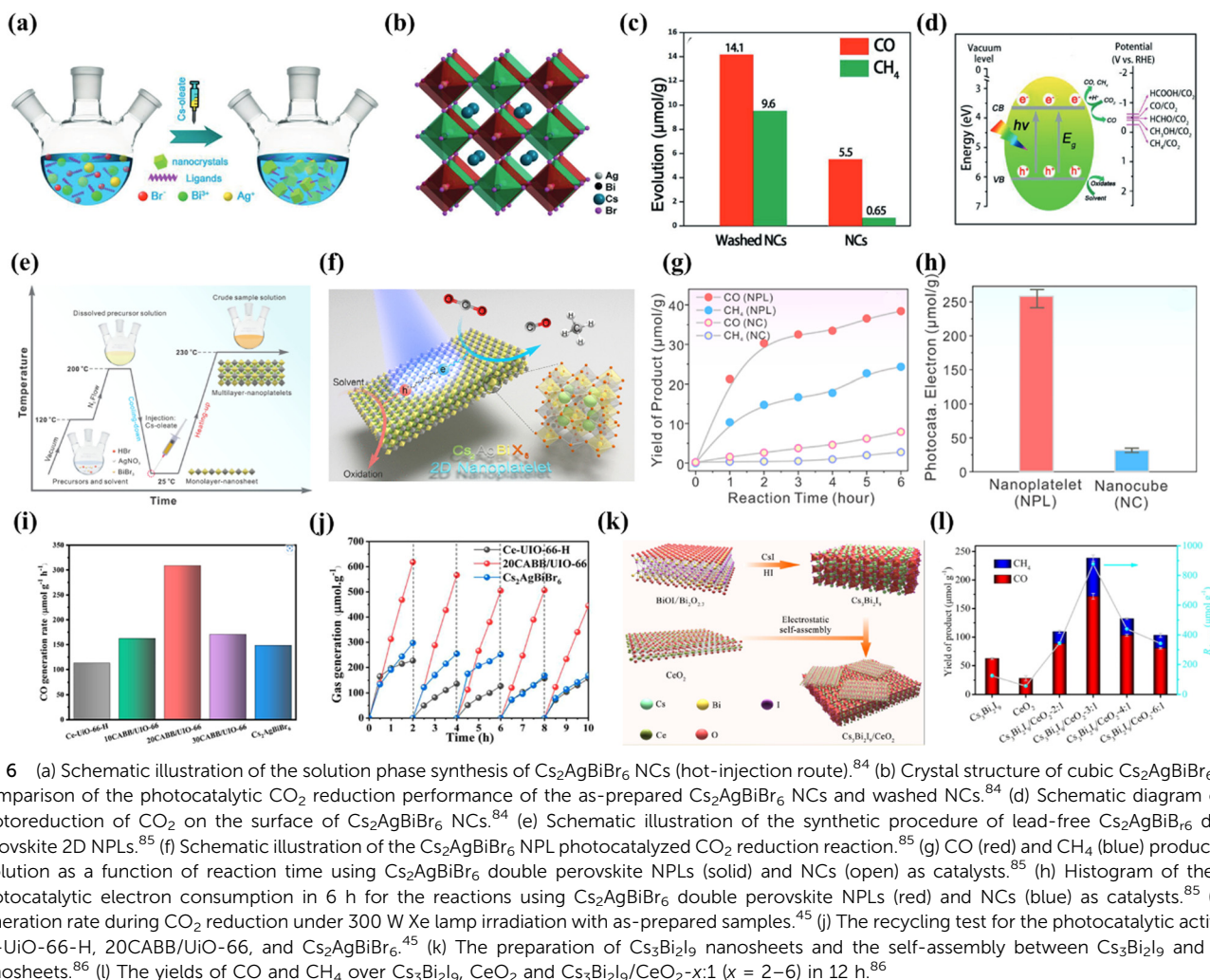
Fig. 6 (a) Schematic illustration of the solution phase synthesis of \text{Cs}_2\text{AgBiBr}_6 NCs (hot-injection route). 84 (b) Crystal structure of cubic \text{Cs}_2\text{AgBiBr}_6 . 84 (c) Comparison of the photocatalytic \text{CO}_2 reduction performance of the as-prepared \text{Cs}_2\text{AgBiBr}_6 NCs and washed NCs. 84 (d) Schematic diagram of the photocatalytic \text{CO}_2 reduction on the surface of \text{Cs}_2\text{AgBiBr}_6 NCs. 84 (e) Schematic illustration of the synthetic procedure of lead-free \text{Cs}_2\text{AgBiBr}_6 double perovskite 2D NPLs. 85 (f) Schematic illustration of the \text{Cs}_2\text{AgBiBr}_6 NPL photocatalyzed \text{CO}_2 reduction reaction. 85 (g) \text{CO} (red) and \text{CH}_4 (blue) product yield evolution as a function of reaction time using \text{Cs}_2\text{AgBiBr}_6 double perovskite NPLs (solid) and NCs (open) as catalysts. 85 (h) Histogram of the total photocatalytic electron consumption in 6 h for the reactions using \text{Cs}_2\text{AgBiBr}_6 double perovskite NPLs (red) and NCs (blue) as catalysts. 85 (i) \text{CO} generation rate during \text{CO}_2 reduction under 300 W Xe lamp irradiation with as-prepared samples. 45 (j) The recycling test for the photocatalytic activity of \text{Ce-UiO-66-H} , 20\text{CABB}/\text{UiO-66} , and \text{Cs}_2\text{AgBiBr}_6 . 45 (k) The preparation of \text{Cs}_3\text{Bi}_2\text{I}_9 nanosheets and the self-assembly between \text{Cs}_3\text{Bi}_2\text{I}_9 and \text{CeO}_2 nanosheets. 86 (l) The yields of \text{CO} and \text{CH}_4 over \text{Cs}_3\text{Bi}_2\text{I}_9 , \text{CeO}_2 and \text{Cs}_3\text{Bi}_2\text{I}_9/\text{CeO}_2 -x:1 (x = 2–6) in 12 h. 86
