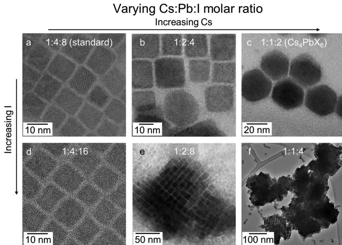
Fig. 2 TEM images of \text{CsPbI}_3 NCs synthesised using HDA-HI at different Cs:Pb:I molar ratios: (a) 1:4:8, (b) 1:2:4, (c) 1:1:2, (d) 1:4:16, (e) 1:2:8, and (f) 1:1:4. All images were taken immediately after synthesis.
