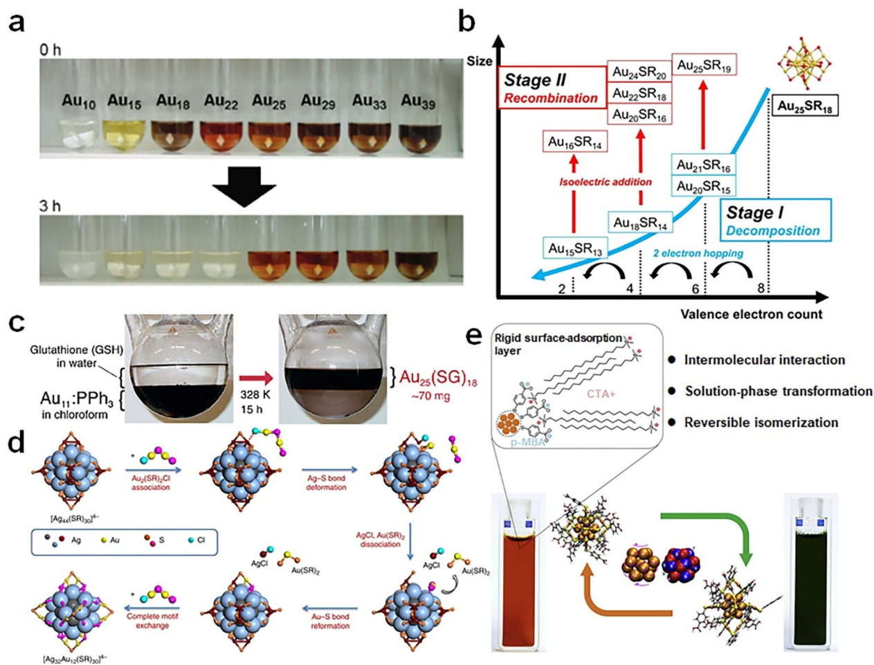
Fig. 5 (a) Aqueous solutions of different \text{Au}_n(\text{SG})_m clusters before (0 h) and after (3 h) the reaction with GSH. Reproduced from ref. 71 with permission from John Wiley and Sons, copyright 2007. (b) Schematic illustration of the etching reaction of water-soluble \text{Au}_{25}(\text{SR})_{18} using excess thiol ligands. Reproduced from ref. 72 with permission from Nature, copyright 2021. (c) Schematic diagram of ligand exchange-induced size conversion from \text{Au}_{11}(\text{PPh}_3)_8\text{Cl}_3 to \text{Au}_{25}(\text{SG})_{18} . Reproduced from ref. 73 with permission from American Chemical Society, copyright 2005. (d) Schematic illustration of the surface motif exchange reaction of [\text{Ag}_{44}(\text{SR})_{30}]^{4-} NCs. Reproduced from ref. 75 with permission from Nature, copyright 2017. (e) Schematic representation of the reversible transformation between the two isomers of [\text{Au}_{25}(\text{p-MBA})_{18}]^- NCs using a cationic surfactant (cetyltrimethylammonium cation, \text{CTA}^+ ). Reproduced from ref. 76 with permission from Cell, copyright 2021.
