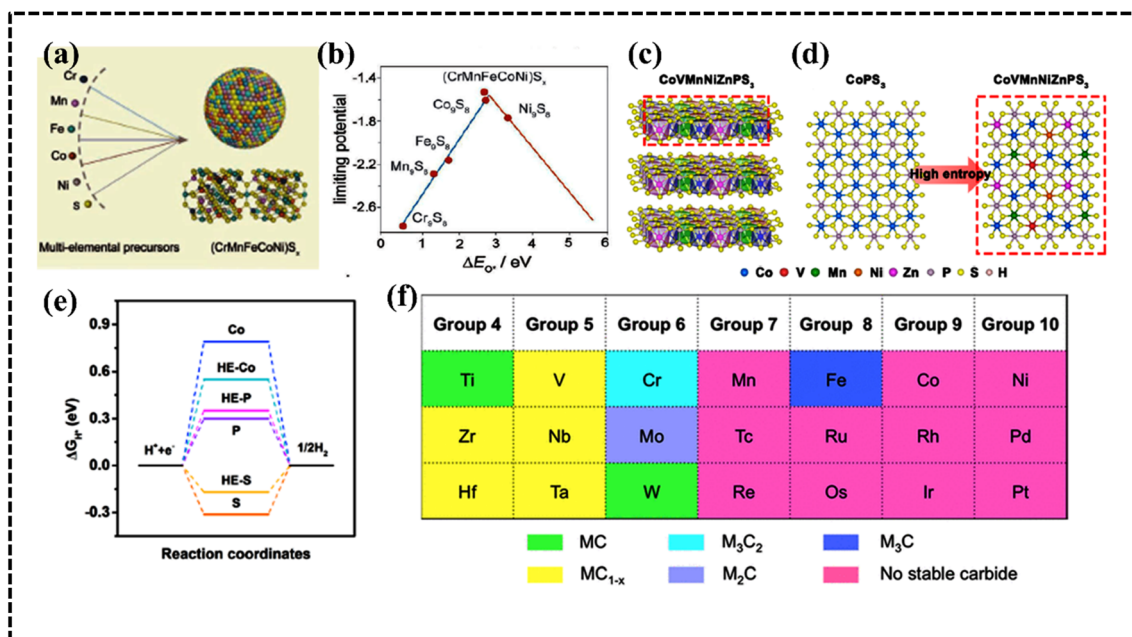
Fig. 10 (a) Schematic demonstrating the structure and activity of high-entropy metal sulfide (\text{CrMnFeCoNi})\text{S}_x nanoparticles. (b) Calculated catalytic activity volcano plot. Reproduced with permission. 147 Copyright 2021, Wiley-VCH. (c) DFT calculation in the edge mode; crystal structure of the monoclinic structure, (d) structural polymorphs of \text{CoPS}_3 and \text{CoVMnNiZnPS}_3 along the top views, and (e) hydrogen evolution reaction free-energy diagram of the corresponding edge sites. Reproduced with permission. 155 Copyright 2022, American Chemical Society. (f) Elements in the synthesized high-entropy carbide (HEC) system. Reproduced with permission. 166 Copyright 2013, American Chemical Society.
