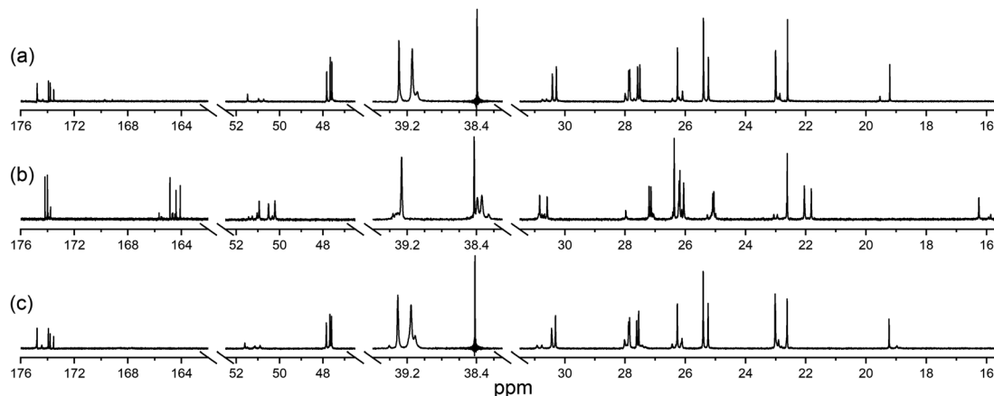
Fig. 1 \{^1\text{H}\} - ^{13}\text{C} NMR spectra from solutions ( \text{D}_2\text{O} ) of (a) 1, (b) Zr(IV) : 1 (1.8 : 1), or (c) Lu(III) : 1 (1.3 : 1). The signal at 38.4 ppm in (a) and (c) is due to a decoupler zero frequency spike.
