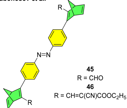
Fig. 18 NBD–azobenzene dimers and trimers reported by Dubonosov et al. 89 in 2001 and Kunz and Wegner in 2020. 90
