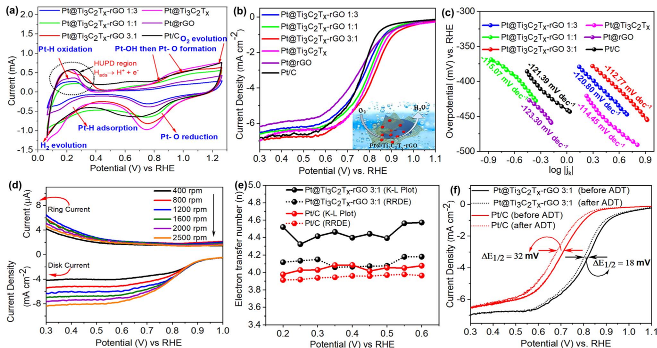
Fig. 4 (a) Cyclic voltammetry curves in O 2 -saturated 0.1 M HClO 4 at a scan rate of 100 mV s -1 , (b) ORR polarization curves of 1600 rpm at 10 mV s -1 , (c) Tafel curves obtained from polarization curves in (b) for Pt@Ti 3 C 2 T x -rGO 1:3, Pt@Ti 3 C 2 T x -rGO 1:1, Pt@Ti 3 C 2 T x -rGO 3:1, Pt@Ti 3 C 2 T x , Pt@rGO, and Pt/C catalysts. (d) RRDE polarization curve of Pt@Ti 3 C 2 T x -rGO 3:1 at different rotation rates; (e) number of electrons transferred by Pt@Ti 3 C 2 T x -rGO 3:1 and Pt/C determined using the K-L plot and RRDE method; (f) accelerated durability test (ADT) for Pt@Ti 3 C 2 T x -rGO 3:1 and Pt/C before and after 10k cycles.
