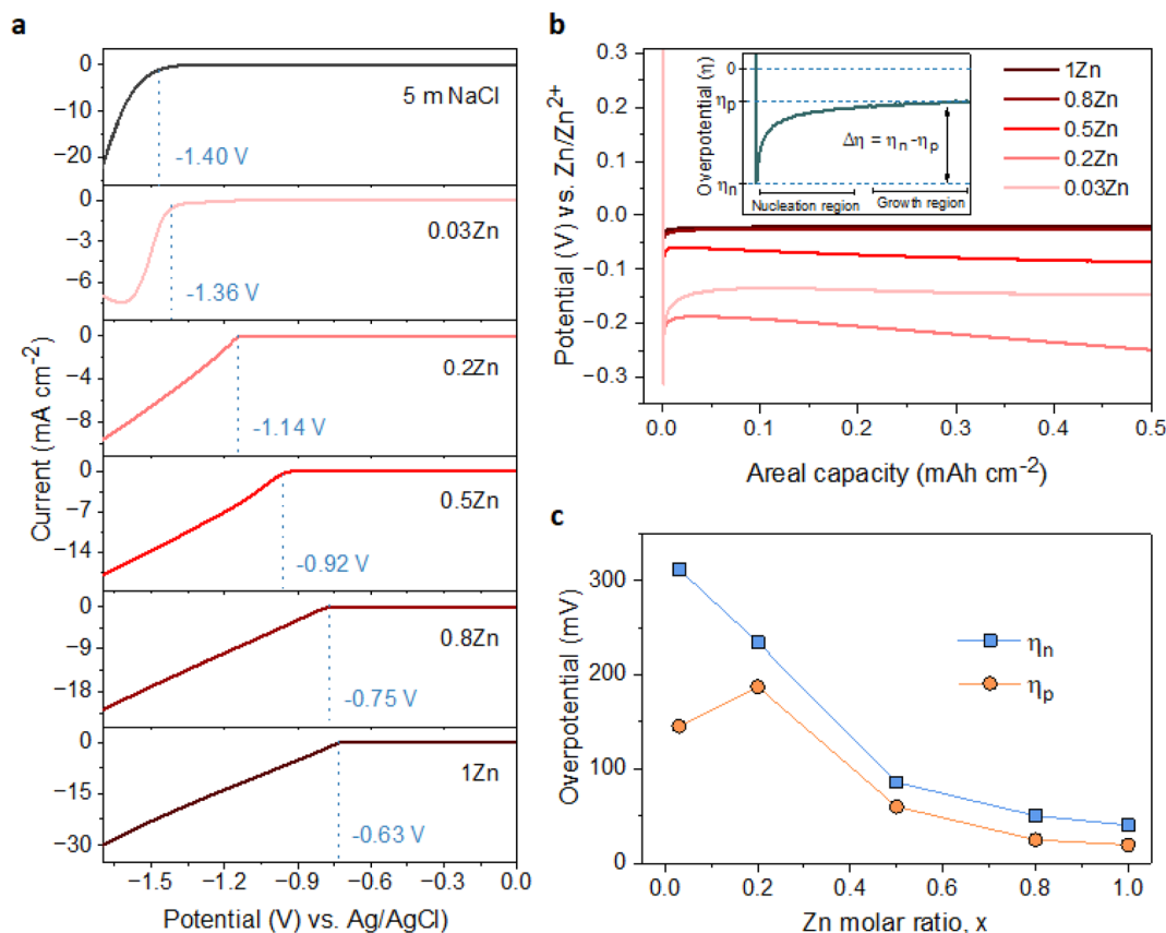
Fig. 2 H_2 evolution and Zn deposition potentials in different WISEs. (a) LSV profiles of different electrolytes at 10 \text{ mV s}^{-1} using a three-electrode system on a Ti substrate. (b) Galvanostatic Zn electrodeposition on Ti in Zn||Ti half cells at 1 \text{ mA cm}^{-2} and 0.5 \text{ mA h cm}^{-2} using different WISEs. Inset: schematic illustration showing nucleation overpotential ( \eta_n ), plateau overpotential ( \eta_p ), and the change in overpotential ( \Delta\eta ). (c) The corresponding change in \eta_n , \eta_p , and \Delta\eta with the Zn molar ratio.
