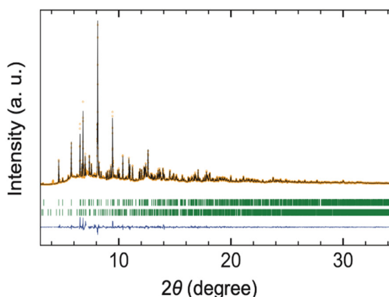
Fig. 2 Rietveld refinement of SXR data collected for LaSI ( \lambda = 0.420201 \text{ \AA} ), adopting the \text{SrI}_2 -type structure with space group Pcab . Orange circles, black lines, and blue lines represent the observed, calculated, and residual intensity, respectively. The green ticks indicate the Bragg reflection positions for LaSI (upper) and \text{La}_{10}\text{OS}_{14} (lower). The weight fraction of \text{La}_{10}\text{OS}_{14} is 13.6(2)%.
