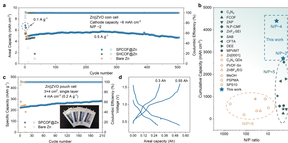
Fig. 7 The performance of Zn metal full cell enabled by SPCOF layer. (a) Cycling performance of Zn||ZVO batteries with different anodes in a 2 M \text{ZnSO}_4 electrolyte at a low N/P ratio of ~2. The Zn thickness is 20 \mu\text{m} , corresponding to a capacity of ~11.7 mA h cm -2 , with a cathode capacity of ~6 mA h cm -2 . (b) Comparison of N/P ratio and cumulative capacity in this work with prior studies. (c) Cycling performance of 3 \times 4 \text{ cm}^2 Zn||ZVO pouch cells. Inset is optical image of as prepared Zn||ZVO pouch cell. (d) Galvanostatic charge–discharge profiles of 0.3 A h and 0.55 A h Zn||ZVO pouch cells.
