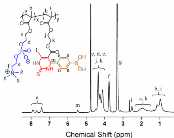
Fig. 2 The chemical structure and 1 H NMR spectrum of zwitterionic PMPD copolymer.
