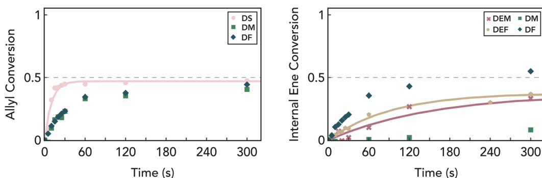
Fig. 5 1 H NMR conversion of allyl (left) and maleate/fumarate (right) in 2 : 1 ratio* photoreactions show a self-limiting reaction for DS, whereas combined maleate/fumarate and allyl consumption exceeds the number of available thiols. Combined with the observation of insoluble solids at long reaction times, this suggests some cross-reaction of allyls and maleates/fumarates is possible at low thiol concentration. *The ratio is allyl : thiol or fumarate/maleate : thiol for DEF and DEM.
