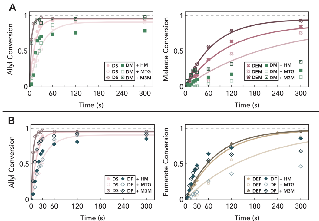
Fig. 4 Functional group conversion as a function of time for 1 : 1 ratios of small molecules with different monothiols show that reaction rate can be tuned by thiol structure. (A) Allyl and maleate conversion of DM plotted with controls DS and DEM (left and right, respectively). (B) Allyl and fumarate conversion of DF plotted with controls DS and DEF (left and right, respectively).
