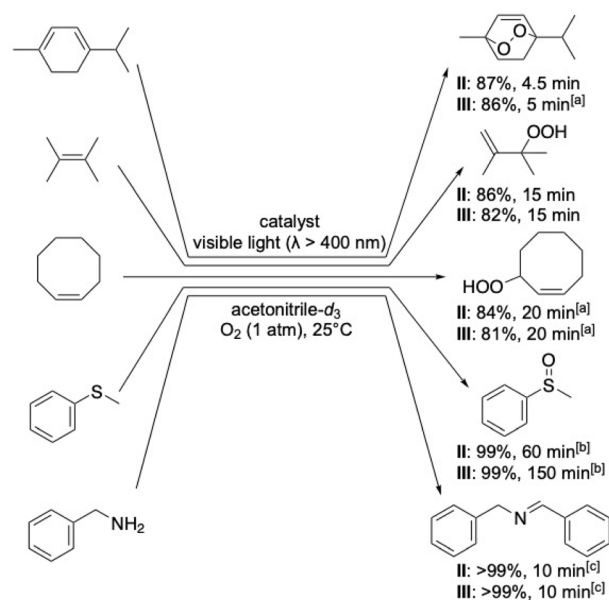
Fig. 6 Aerobic oxidation of various substrates using hybrids II and III under visible light irradiation. Reaction conditions: substrate (0.1 mmol), catalyst ( II and III : 0.003 \mu\text{mol} ), acetonitrile- d_3 (0.7 mL), visible light ( \lambda > 400 \text{ nm} ), 25 ^{\circ}\text{C} , \text{O}_2 (1 atm). Product yields and conversion were determined by ^1\text{H} NMR using anisole as an internal standard. a Catalyst (0.03 \mu\text{mol} ). b Acetonitrile/water (2 mL, 95/5, v/v). GC yields using dodecane as an internal standard. c Acetonitrile (2 mL). GC yields using dodecane as an internal standard.
