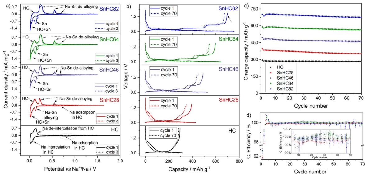
Fig. 1 (a) Cyclic voltammograms at 0.1 mV s -1 for Sn/HC electrodes with different Sn : HC weight ratio. (b) Voltage profile during galvanostatic cycling at 50 mA g -1 (1 st cycle) and 100 mA g -1 (70 th cycle) and corresponding (c) cycling stability in terms of charge (de-sodiation) capacity and (d) coulombic efficiency. Tests conducted at 25 °C within the 0.01–1.5 V range. Electrolyte: 1 M NaPF 6 in diglyme.
