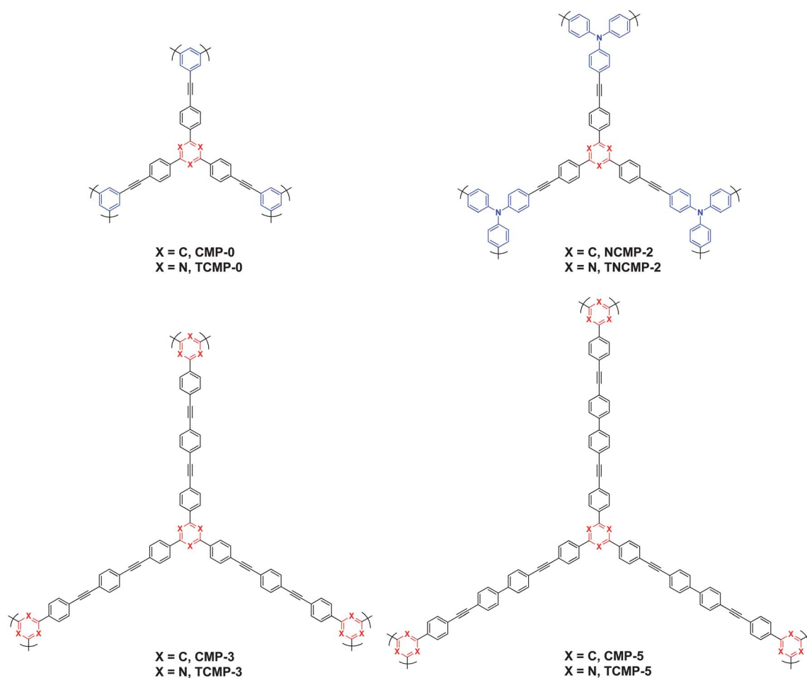
Scheme 1 Representative molecular structures for TCMP networks and the corresponding CMPs.
