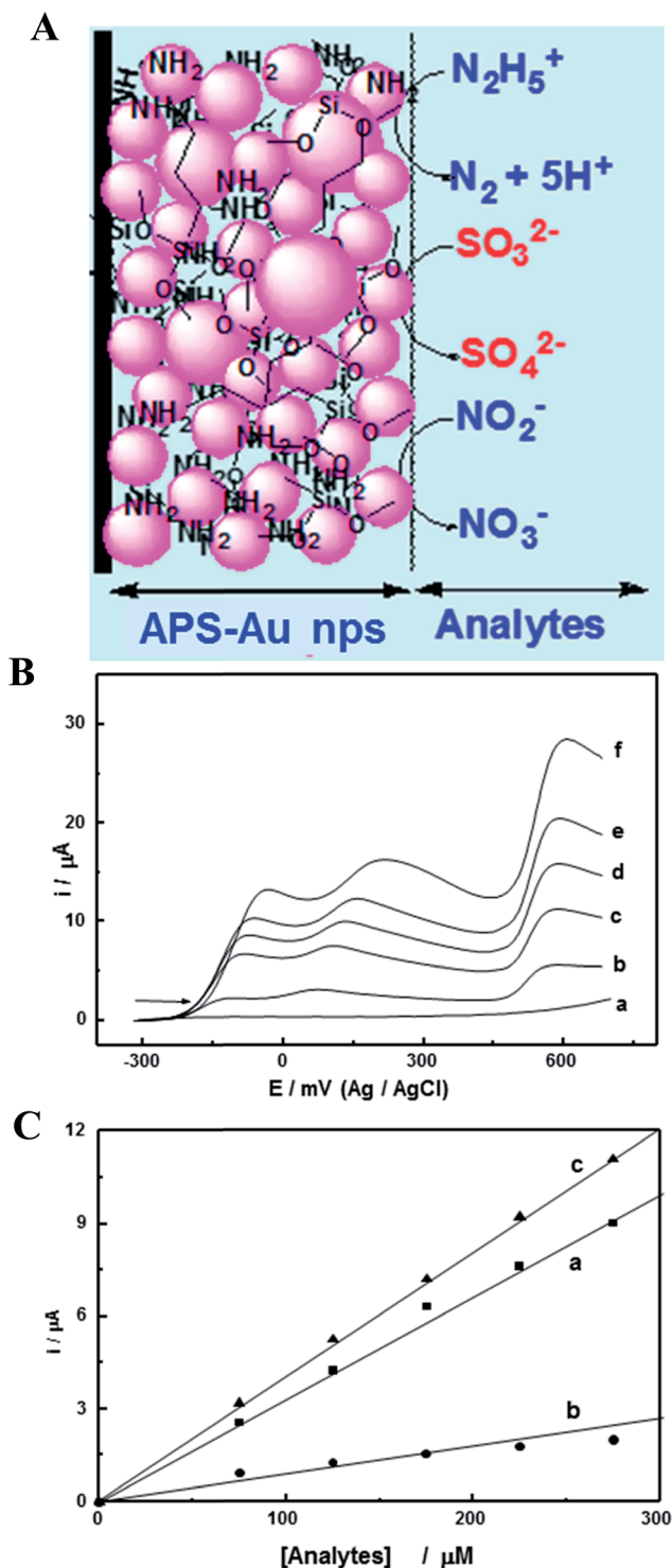
Fig. 7 (A) Schematic representation of an APS-Au NPs modified GC electrode and simultaneous electrocatalytic oxidation of N_2H_4 , SO_3^{2-} and NO_2^- . (B) LSVs recorded at APS-AuNPs modified GC electrode for the mixture of N_2H_4 , SO_3^{2-} and NO_2^- with the successive addition of concentrations in 0 (a), 200 \mu M (b), 300 \mu M (c), 400 \mu M (d), 500 \mu M (e) and 600 \mu M (f) in 0.1 MPBS (pH 7.2). (C) Corresponding calibration plots for N_2H_4 (a), SO_3^{2-} and NO_2^- (c). Reproduced with permission from ref. 129 © 2007 Elsevier.
