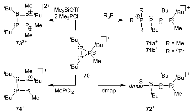
Scheme 28 Diverse reactivity of cation 52 + in the reaction with a series of nucleophiles such as \text{Me}_2\text{PCL} , \text{MePCL}_2 , \text{R}_3\text{P} and \text{dmap} (4-(dimethylamino)-pyridine).
