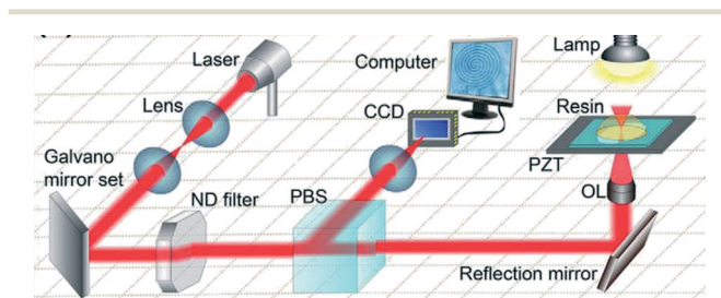
Fig. 14 Schematic femtosecond laser direct writing system. The femtosecond laser focused by a lens (1.4, oil immersion used here). The laser scanning path was precisely controlled by computer according to the pre-programmed structures from the bottom slice to the upside slice until the entire 3D structure is achieved. The imaging system using a charge couple device (CCD) is useful both for optical adjustment and for in situ fabrication monitoring. PBS: polarization beam splitter; OL: objective lens; PZT: piezoelectric transducer. 75 (Copyright 2015 Elsevier).
