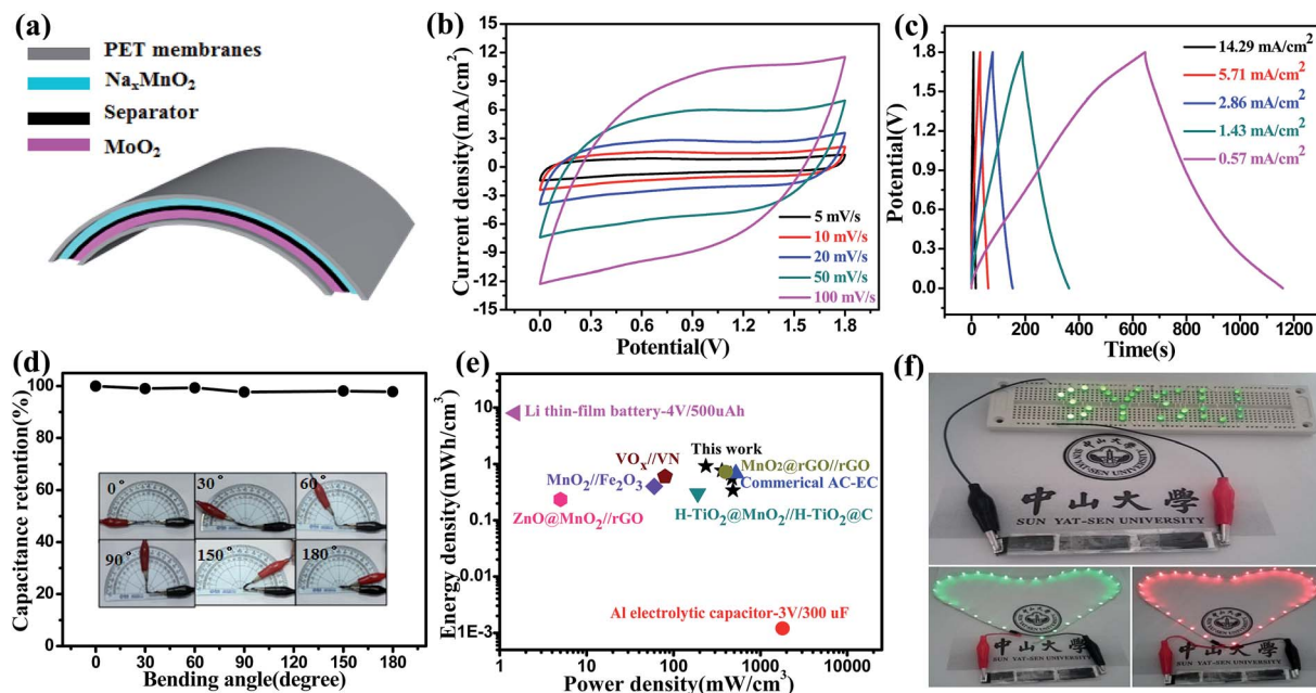
Fig. 5 (a) A schematic illustration of the structure of a flexible \text{Na}_{0.44}\text{MnO}_2/\text{CC} // \text{MoO}_2/\text{CC} ASC with two electrodes separated by the TF45 (NKK) membrane (separator); (b) CV curves of the ASC at different scan rates; (c) GCD curves of the ASC at different current densities; (d) stability performance of the ASC collected at different bending angles (the inset shows the flexibility under the different bending angles); (e) Ragone plots of the \text{Na}_{0.44}\text{MnO}_2/\text{CC} // \text{MoO}_2/\text{CC} ASC device. The values reported in the literature for other ASC devices are added for comparison; (f) a SYSU logo consisting of 32 green LEDs and a piece of commercial red or green LED soft rope light powered by the assembled ASCs with three in series.
