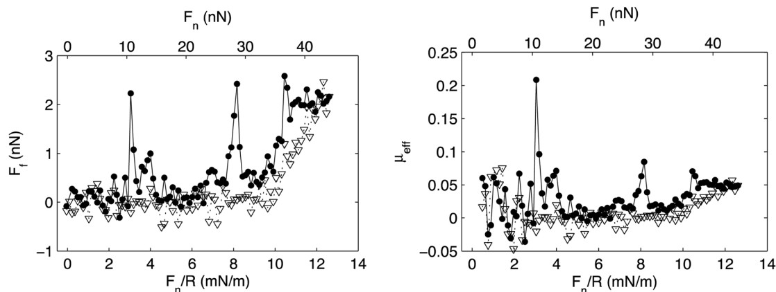
Fig. 10 Left panel: Friction force, F_f , vs. load, F_n , F_n/R , and F_n , between a mica and a silica surface coated with the cationic polyelectrolyte PMAPTAC across a 1 cmc SDS solution. Filled and unfilled symbols represent data obtained upon loading and unloading, respectively. Right panel: Effective friction coefficient, \mu_{\text{eff}} , vs. load. The symbols correspond to the same experimental conditions as described for the left panel. Reproduced from ref. 35 with permission from the Royal Society of Chemistry.
