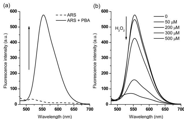
Fig. 2 Fluorescence spectra ( \lambda_{\text{ex}} = 460 nm) of ARS only (50 \mu M), ARS–PBA (ARS, 50 \mu M; PBA, 200 \mu M, 15 min) (a) and then addition of \text{H}_2\text{O}_2 (50, 200, 300, 500 \mu M), respectively for 60 min (b). The data was obtained in 1/15 M PBS buffer with 2.0 mM CTAB solution at 25 ^{\circ}\text{C} .
