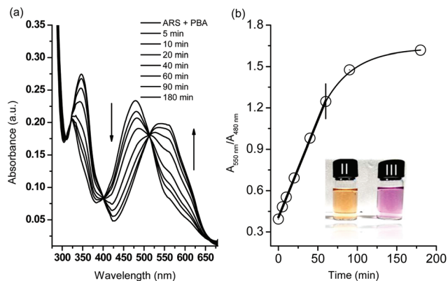
Fig. 1 (a) UV-Vis absorption spectra for ARS only (50 \mu M), ARS–PBA (ARS, 50 \mu M; PBA, 200 \mu M) and then addition of \text{H}_2\text{O}_2 (500 \mu M, 5, 10, 20, 40, 60, 90, 180 min). (b) The data was obtained in 1/15 M PBS buffer with 2.0 mM CTAB in solution at 25 ^{\circ}\text{C} .
