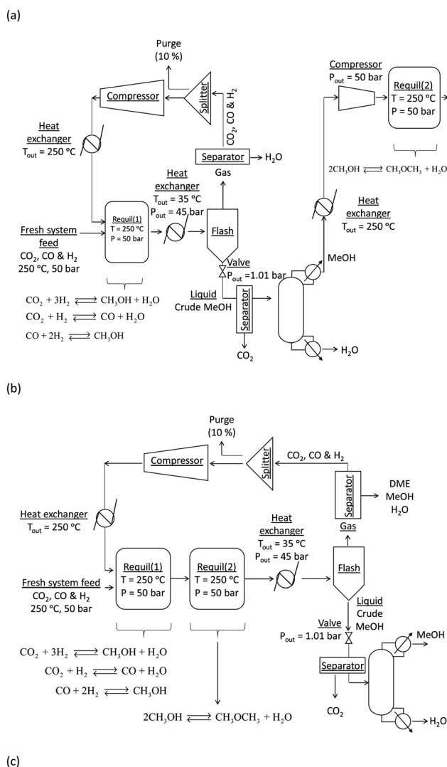
Fig. 4 Schematics of process layouts for direct and indirect DME synthesis from syngas.
