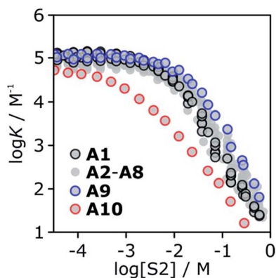
Fig. 16 Association constants ( \log K/\text{M}^{-1} ) for formation of the 6:13 complex as a function of alcohol concentration (S2) in n -octane (S1) at 298 K. Data highlighted are 1-octanol A1 (black), 3-ethyl-3-pentanol A9 (blue) and trifluoromethyl-2-octanol A10 (red).
