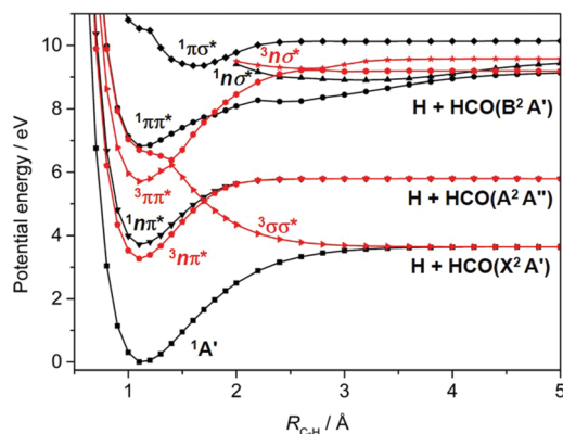
Fig. 3 Rigid body singlet (in black) and triplet (in red) PECs for HCHO plotted as a function of R_{C-H} for planar geometries, with the rest of the nuclear framework maintained at its ground state equilibrium geometry.
