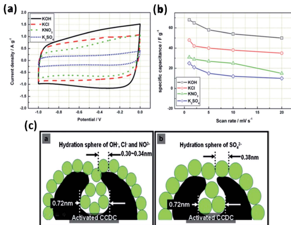
Fig. 8 (a) Cyclic voltammograms of activated CCDC supercapacitors in the aqueous electrolytes 0.5 M K_2SO_4 , 2 M KCl, 1 M KNO_3 and 6 M KOH (20 mV s -1 ) and (b) the specific capacitance of the supercapacitor at different scan rates. (c) Schematic diagram of the relationship of hydration sphere ions and pores. This figure has been adapted from ref. 115 with permission from Elsevier.
